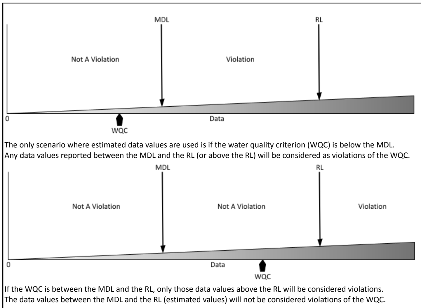
Figure 1. Two scenarios involving the use of estimated data for determining water quality criteria violations related to WQC, MDLs, and RLs.
